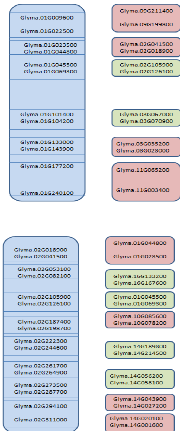
Figure S1: Segmental duplication of each chromosome of soybean. Length of segment (not to scale). Duplication in green colour- direct duplication; in red colour- reverse duplication
