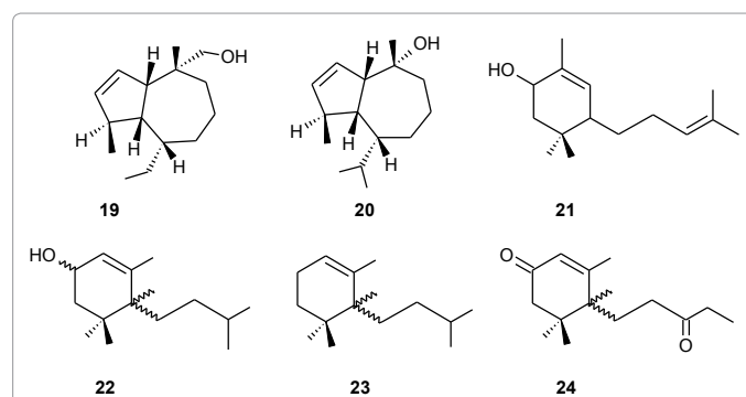
Figure 4: Structures of guai-2-en-10α-methanol (19) and guai-2-en-10α-ol (20), 2,5,5-trimethyl-4-(4'-methyl-3'-pentenyl)-2-cyclohexen-1-ol (21), 4-isopentyl-3,4,5,5-tetramethyl-2-cyclohexen-1-ol (22, two diastereoisomeric compounds), 6-isopentyl-1,5,5,6-tetramethyl-1-cyclohexene (23), and 3,4,5,5-tetramethyl-4-(3'-oxopentyl)-2-cyclohexen-1-one (24).
