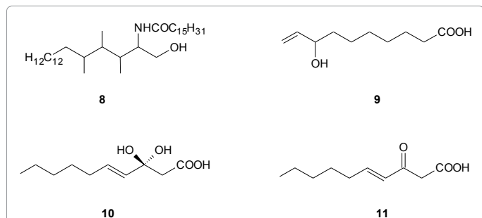
Figure 2: Structures of N -palmitoyl-2-amino-1,3,4,5-tetrahydrooctadecane (8), 8-hydroxy-9-decenoic acid (9), 3,3-diol-4-decenoic acid (10), and 3-oxo-4-decenoic acid (11).
