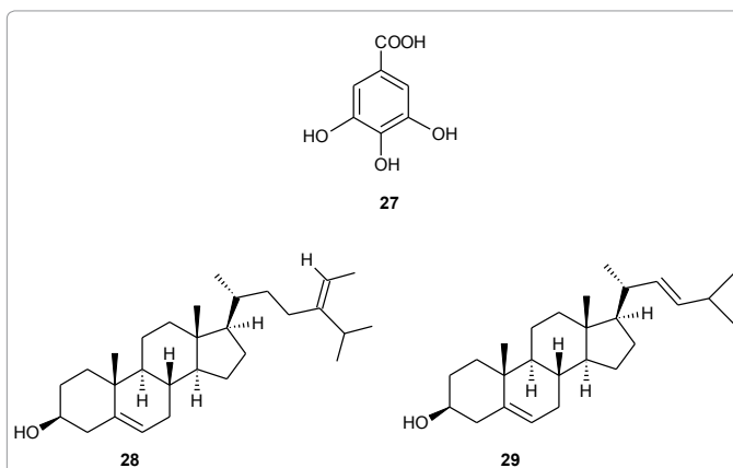
Figure 6: Structures of gallic acid (27), 24-nor-22-dehydrocholesterol (28) and isofucosterol (29).
