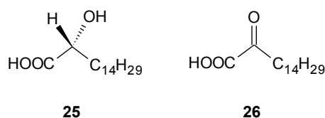
Figure 5: Structures of 2(R)-hydroxy-hexadecanoic acid (25) and 2-oxo-hexadecanoic acid (26).
