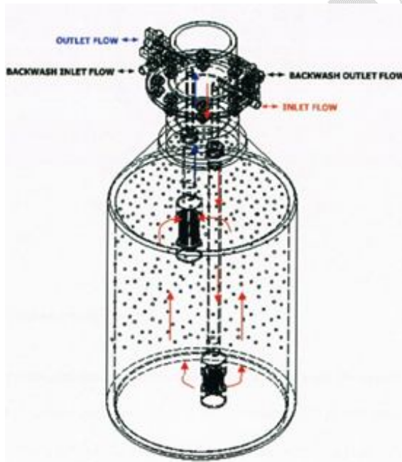
Figure 5a: Filtration mode.
