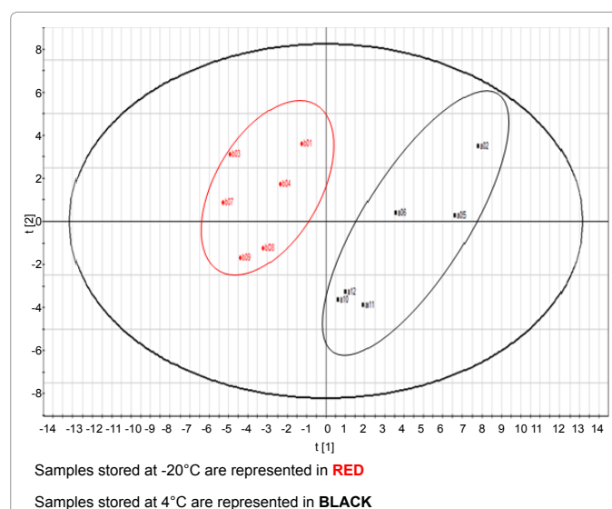
Figure 5a: PCA plot for all 12 samples (six stored at 4°C and six stored at -20°C). All the observations were within the Hotelling T 2 's 95% confidence. The X-axis represented t [1] which shows score t [1] for Principal component 1 (PC1) showing maximum variation in the dataset. The Y-axis represented t [2] which represents score t [2] for Principal component 2 (PC2) showing maximum variation not seen from just PC1. ZIC HILIC column (2.1 mm × 150 mm × 5 μm) at flow rate of 0.2 mL min -1 was used to acquire the data. The mobile phases used were- 50 mM ammonium acetate: acetonitrile (95:5 v/v) and 50 mM ammonium acetate: water: acetonitrile (50:45:5 v/v). The gradient program is described in Table 1.
