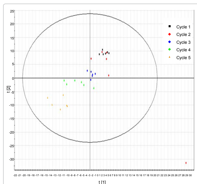
Figure 7: PLS-DA plot showing variation between the samples analyzed after each freeze and thaw cycle. Five freeze and thaw cycles showed variation within 95% confidence of Hotelling T2 with one outlier seen in freeze thaw cycle 2. The X-axis represented t [1] which shows score t [1] for PC1 showing maximum variation in the dataset. The Y-axis represented t [2] for PC2 showing maximum variation not seen from just PC1. The coloured key represents each freeze and thaw cycle after which the samples were analyzed.
