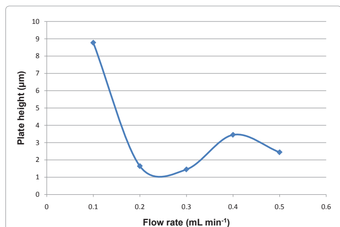
Figure 3a: Van Deemter plot for Sequant ZIC HILIC column (5 µm, 150 mm × 2.1 mm i.d.), Column temperature: 40°C; UV: 254 nm. The mobile phases used were- 50 mM ammonium acetate: acetonitrile (95:5 v/v) and 50 mM ammonium acetate: water: acetonitrile (50:45:5 v/v). The gradient program is described in Table 1.
