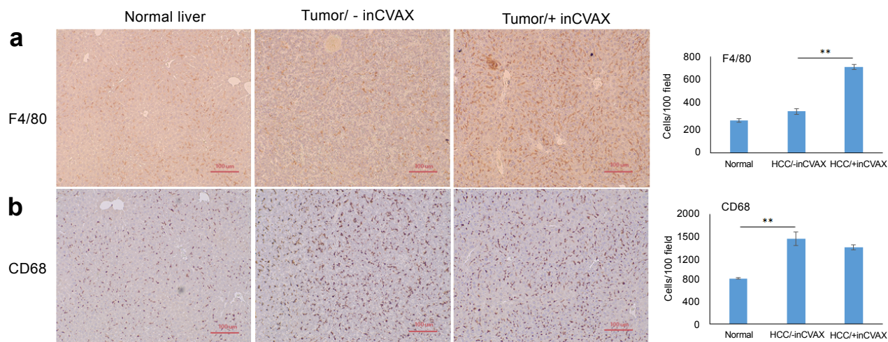
Figure 5: Effect of inCVAX on macrophage infiltration into tumors. Immunohistochemical staining of F4/80 (a) and CD68 (b) were performed in normal liver tissues from control syngeneic wild type C57BL/6 mice and tumor tissues from large HCC-bearing mice with and without inCVAX. Tumor progression led to slight increase of F4/80 + macrophages into tumor tissue. Additionally significant increase of tumor-infiltrating F4/80 + macrophages was detected in HCC-bearing mice received inCVAX. In contrast to F4/80 + macrophages, more CD68 + macrophages were stained in the liver of normal mice. Tumor growth dramatically drove more CD68 + macrophages infiltration into tumors. inCVAX slightly suppressed this trend. The average liver- or tumor-infiltrated T cells per 100 fields were calculated. 100 × magnification, n=3, *p<0.05, **p<0.01, error bars represent mean ± SDs.
