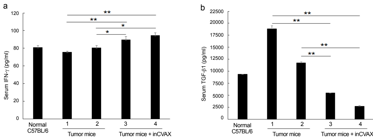
Figure 3: inCVAX modulates levels of serum cytokines in tumor-bearing mice. Blood was harvested from tumor-bearing mice with or without inCVAX and used to isolate serum. The level of cytokine IFN- \gamma (a) and TGF- \beta 1 (b) were measured with ELISA in duplicate. n=2, *p<0.05, ** p<0.01, error bars represent mean \pm SDs. inCVAX led to significant increase of IFN- \gamma , but reduction of TGF- \beta 1 in large HCC-bearing mice.
