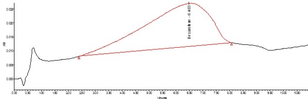
Figure 3b: Bexarotene in mobile phase (Buffer: ACN:80:20 V/V), pH 3.0.
