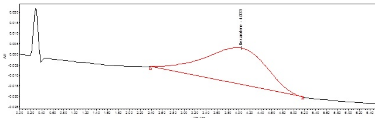
Figure 3c: Bexarotene in mobile phase (Buffer: ACN:70:30 V/V), pH 3.0.
