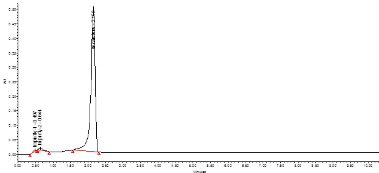
Figure 3d: Bexarotene in mobile phase (Water: AC:70:30 V/V), pH 3.0, 0.25 mL TFA.
