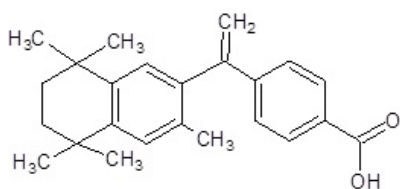
Figure 1a: The structures of Bexarotene and its impurities. Bexarotene. 4-[1-(3,5,5,8,8-pentamethyl-6,7-dihydronaphthalen-2-yl)ethenyl]benzoic acid.
