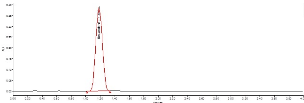
Figure 3g: Bexarotene standard chromatogram in final conditions.
