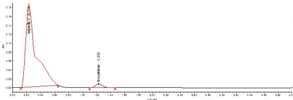
Figure 3f: Bexarotene capsules degradation with 1 M NaOH at Room temperature for 24 h.
