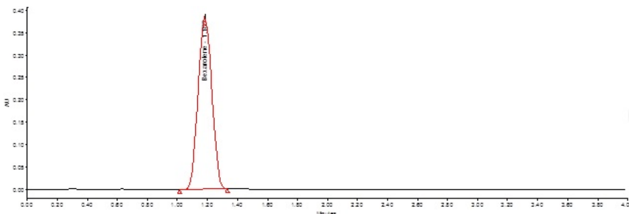
Figure 3h: Bexarotene sample chromatogram in final conditions.
