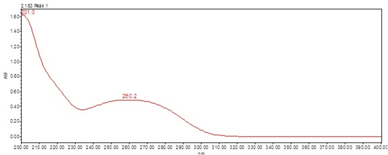
Figure 2: Typical UV Spectrums of Bexarotene and all impurities. Peak-1: imp-1, Peak-2: imp-2, Peak-3: Bexarotene, Peak-4: imp-3 and Peak-5: imp-4.
