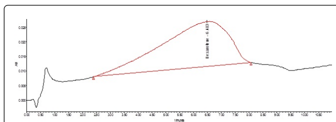
Figure 3a: Bexarotene in mobile phase (Buffer: ACN:60:40 V/V), pH 7.5.
