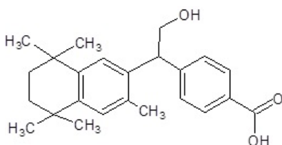
Figure 1b: The structures of Bexarotene and its impurities. 4-[1-(3,5,5,8,8-pentamethyl-6,7-dihydronaphthalen-2-yl)ethyl hydroxy]benzoic acid.
