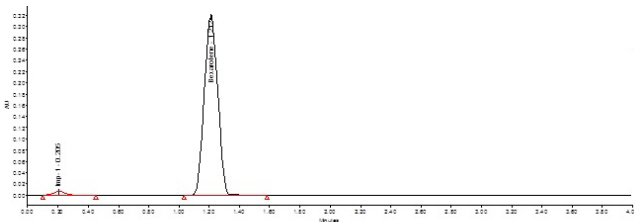
Figure 3e: Bexarotene in mobile phase (Water: ACN:70:30 V/V), pH 3.0, 1.0 mL TFA.
