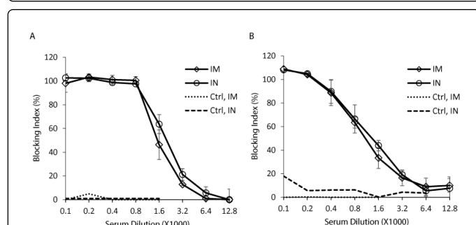
Figure 3: Blocking of NoV GII-4 VLP binding to the HBGA receptors by immune mouse sera. Group wise pooled (five mice/group), two-fold diluted sera of mice immunized by IM or IN route with a NoV vaccine candidate containing 10 µg GII-4 VLPs were assayed for blocking activity. Corresponding control group serum was used as a non-specific blocking control. (A) Blocking of GII-4 VLP binding to human secretor positive saliva type A. (B) Blocking of GII-4 VLP binding to the H-t-3 synthetic HBGA. The blocking index (%) was calculated as 100\% - (\text{OD wells with serum} / \text{OD wells without serum}) \times 100\% . Results are shown as the mean blocking index of duplicate wells with similar results from a minimum of two independent experiments.
