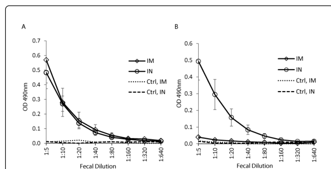
Figure 2: NoV GII-4-specific mucosal antibody responses in BALB/c mice. Mice were immunized twice with a NoV vaccine candidate containing 10 µg GII-4 VLPs. Intestinal IgG (A) and IgA (B) antibodies were analyzed from 10% fecal suspensions of IM and IN immunized mice (solid lines) or the control mice (dashed lines). Fecal samples of five mice/experimental group were pooled for analysis. Shown are mean ODs with the standard errors of the mean (SEM) of two independent experiments.
