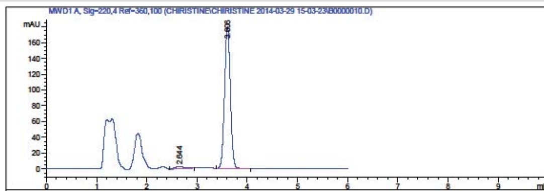
Figure 6: HPLC Chromatogram of QTF in Seroquel® tablets.
