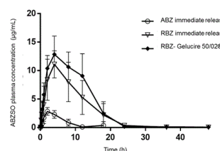
Figure 9: Comparative (mean \pm SD) plasma profiles for ABZSO after the oral administration of one ABZ-based immediate release formulation given orally at 25 mg/kg, one RBZ immediate release formulation and RBZ-Gelucire 50/02' administered orally at 20 mg/kg.
