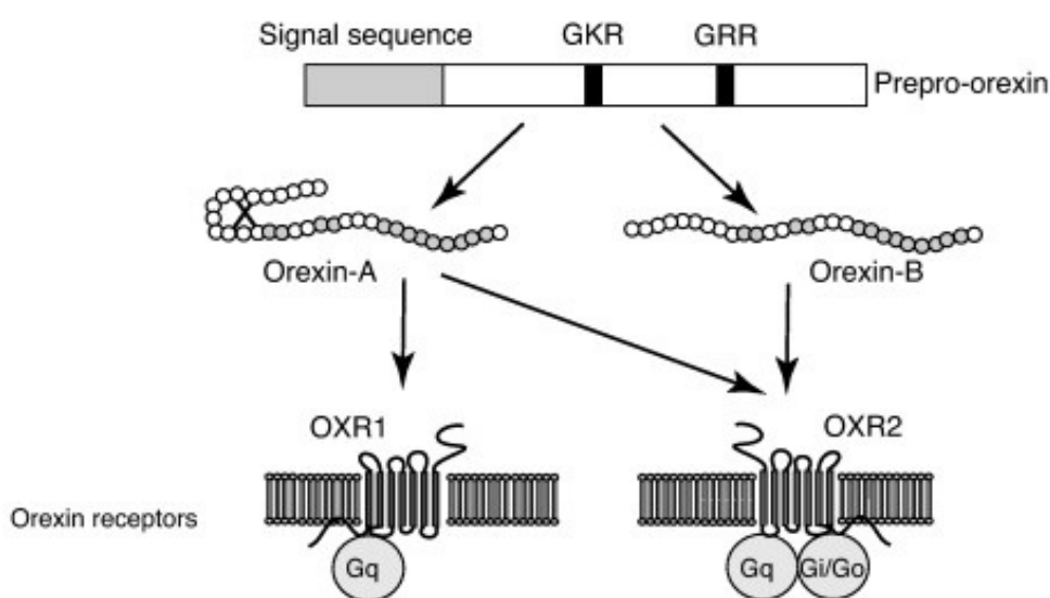
Figure 1: Orexin A and orexin B are derived from a common precursor peptide, prepro-orexin. The actions of orexins are carried out thanks to two receptors that have G protein denominated OXR-1 and OXR-2 receptors. OXR-1 is selective for orexin A, while OXR-2 shows similar affinity for both orexin A and orexin B. OXR-1 is coupled to the Gq subclass of heterotrimeric G proteins, while OXR-2 couples to Gi/o and/or GQ cell lines.
