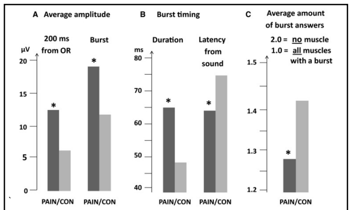
Figure 3: Average for all eight startle sound events together, including all six muscles, for: (A) Mean amplitude during 200 ms from OR-activity-start and during burst, (B) Burst duration and -latency (ms) from sound to muscle-activity-start ( \geq 10 \mu V ), (C) Average amount of bursts:-mean of 1.0=all muscles burst (peak \geq 10 \mu V ) and 2.0=no muscle had burst (peak \geq 10 \mu V ) in any of the eight stimuli. PAIN versus CON showed significant differences (star*). [OR, orbicularis oculi, ref. 2].
