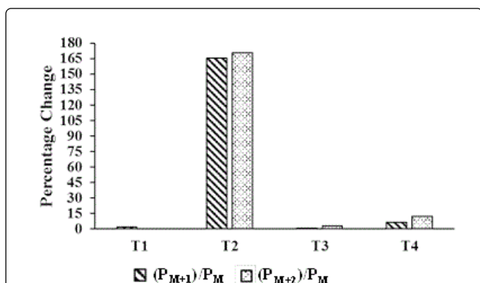
Figure 5: Percent change of isotopic abundance ratios of P_{M+1}/P_M and P_{M+2}/P_M in the biofield energy treated resorcinol as compared to the control sample.
