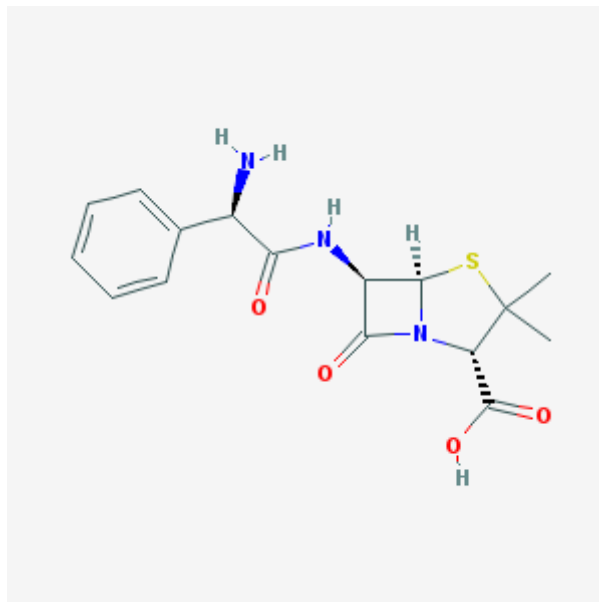
Figure 1:Ampicillin
