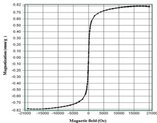
Figure 3: Magnetization Curves of magnetite nanoparticles synthesized at 250°C.
