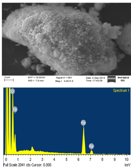
Figure 2: SEM and EDS images of magnetite nanoparticles at 250°C.
