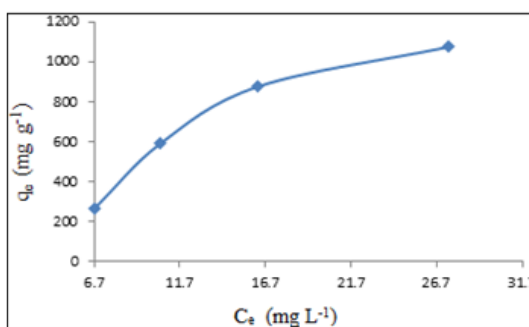
Figure 4: Plot of q_e vs. C_e for adsorption of Cr(VI) on to Fe 3 O 4 nanoparticles at pH 8.2, 0.01 g Fe 3 O 4 .
