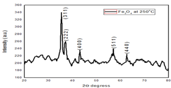
Figure 1: X-ray diffraction of magnetite nanoparticles at 250°C.
