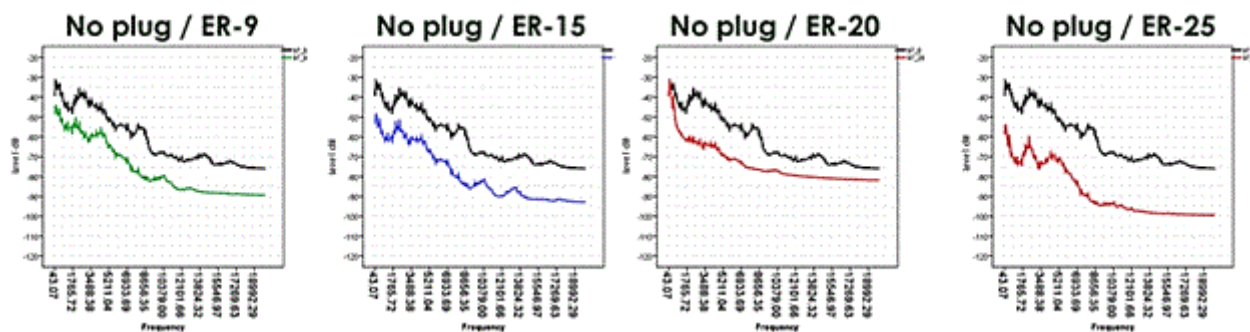
Figure 5: Frequency responses of MEPs compared to no plug condition as measured in KEMAR at 97 dB presentation level.
