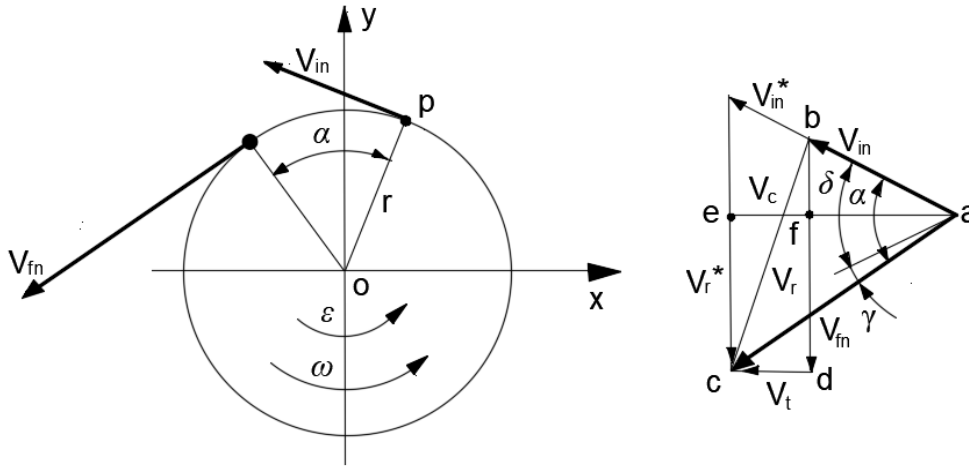
Figure 1: Vectorial velocity polygon of the rotating object about a fixed point.
