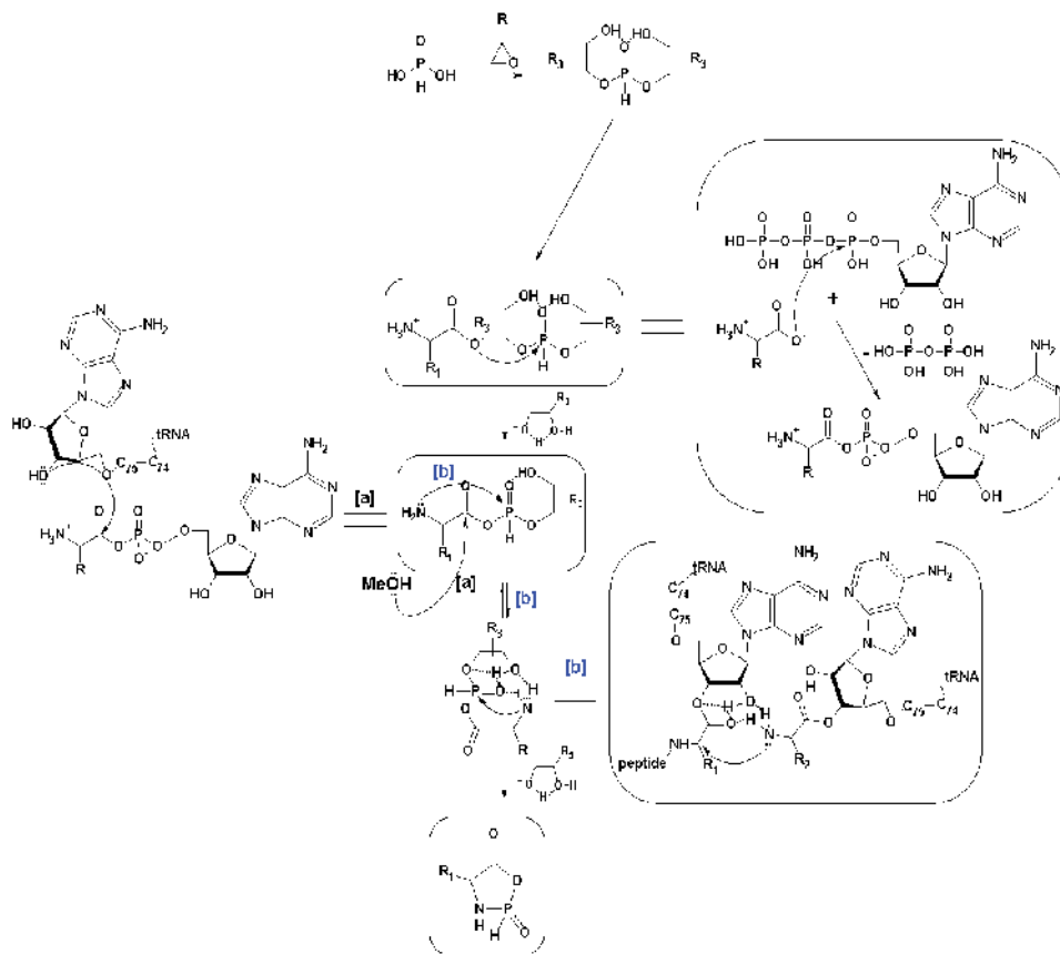
Figure 4: Comparison between the different stages of our proposed ribozyme-mimetic reaction with the important points of peptide synthesis proceeds on the ribosome. As it can be seen from the figure, a considerable analogy is described between them.
