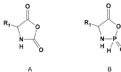
Figure 2: Structures of urethane N-carboxy anhydride (UNCA) A, and 4-alkyl 2,5-dioxo 1,3-oxaza 2-H 2-phospholane B.
