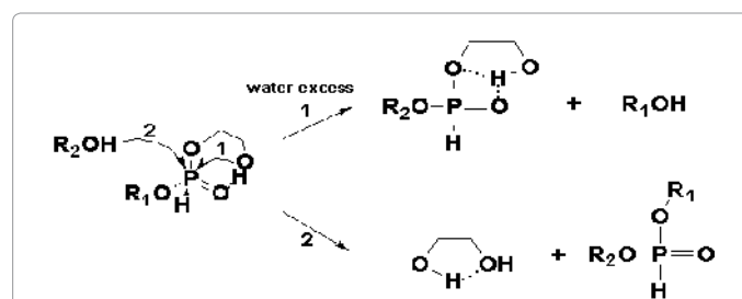
Figure 5a: Scheme of the mono-ol leaving (pathway 1) and diol leaving (pathway 2), accelerated in the presence of the vicinal hydroxyl group, during the reaction of alcoholysis of H-phosphonate diester. In the presence of water excess (pathway 1), due to the impairing of the intramolecular hydrogen bond between the cis-vicinal 2-OH group and the phosphoryl oxygen atom, by the creation of intermolecular hydrogen bonds (between the cis-vicinal 2-OH group and H 2 O from the one side, and between the phosphoryl oxygen atom and H 2 O from the another side) the nucleophilicity of the cis-vicinal 2-OH group is increased and leads to the intramolecular nucleophile attack, supported by the mono-ol (ester alcohol) leaving and following with the ring opening by the intermolecular nucleophile attack by another alcohol molecule. In this case the cis-vicinal 2-OH group plays a role as nucleophile catalyst. Since the reaction proceeds in aprotic solvent (pathway 2), due to the electrophile assistance of the cis-vicinal 2-OH group by its intramolecular hydrogen bonding with the phosphoryl oxygen atom, the electrophilicity of the phosphorus atom bonded with latter and its susceptibility to the intermolecular nucleophile attack is increased, which cause the ester exchange (transesterification) reaction, accompanied with the 1,2-diol leaving [45]. In that case the cis-vicinal 2-OH group plays a role as electrophile catalyst.
