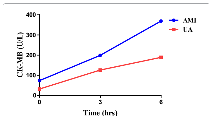
Figure 9: The representative time course of CK-MB level in patients suffering from AMI & UA during first six hours after admission.
