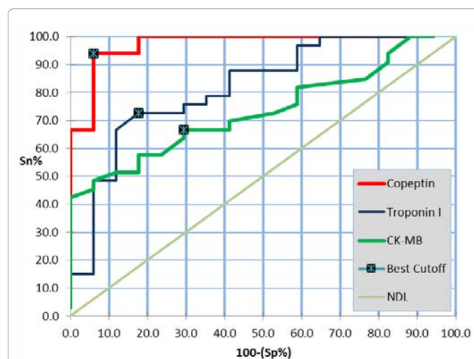
Figure 10: The ROC curve of copeptin, cTn-I and CK-MB at admission time.
