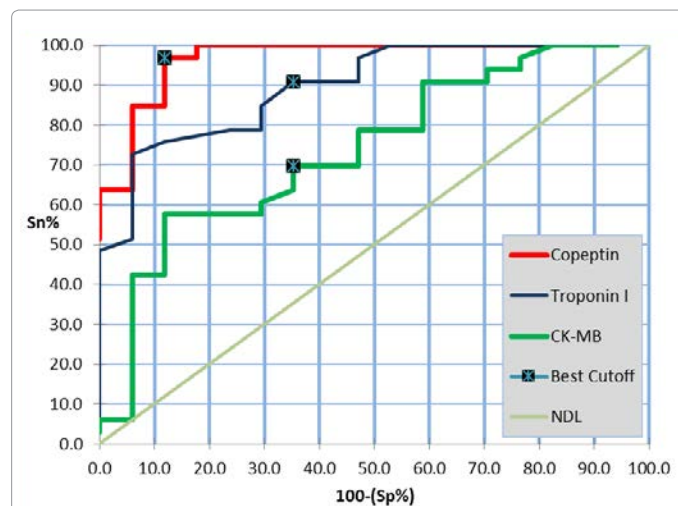
Figure 11: The ROC curve of copeptin, cTn-I and CK-MB at three hours.
