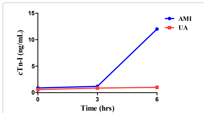
Figure 8: The representative time course of cTn-I level in patients suffering from AMI & UA during first six hours after admission.
