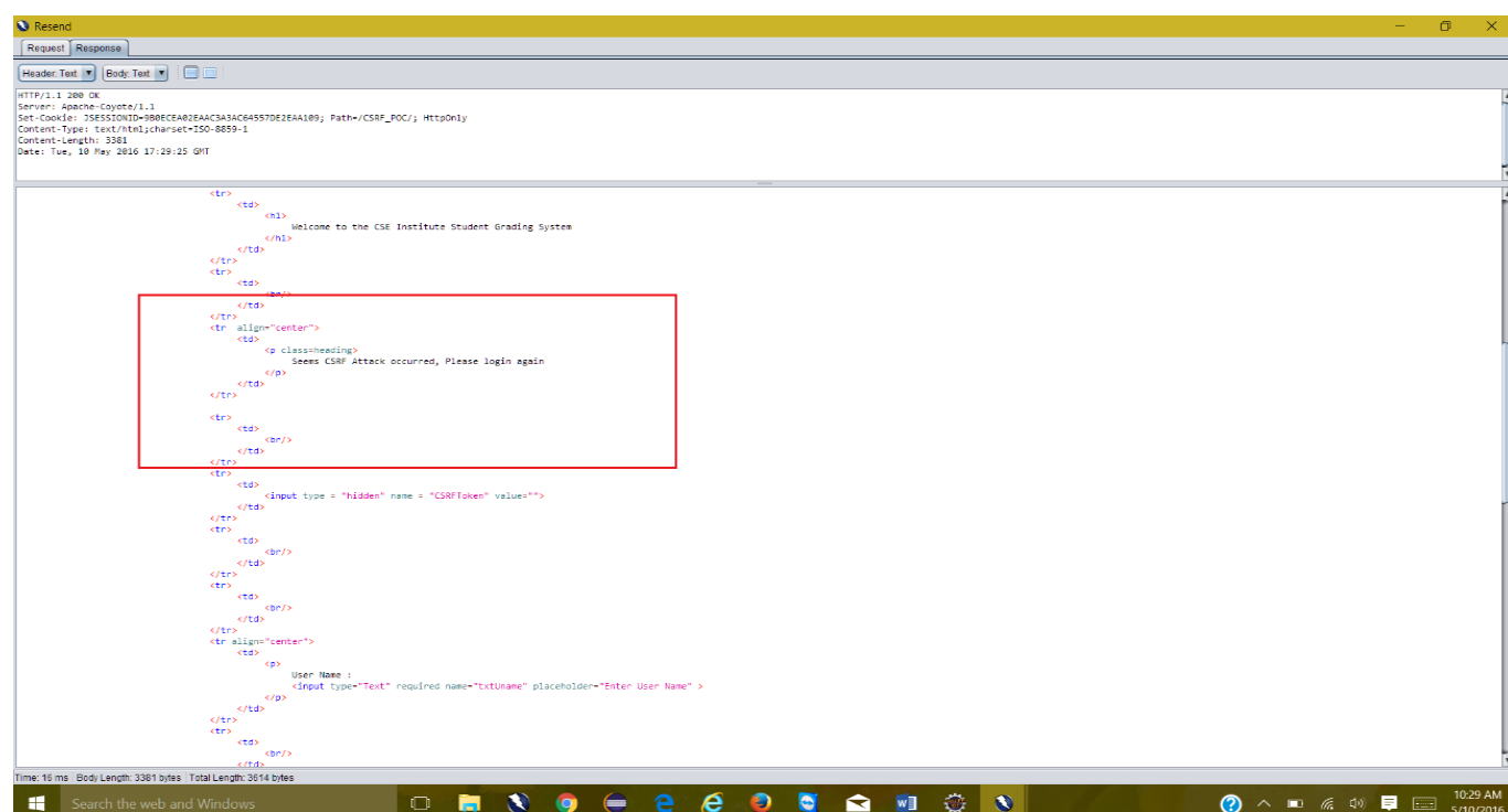
Figure 8: Diagram of representation of Response returned by Server for forged HTTP Request on ZAP Proxy.
