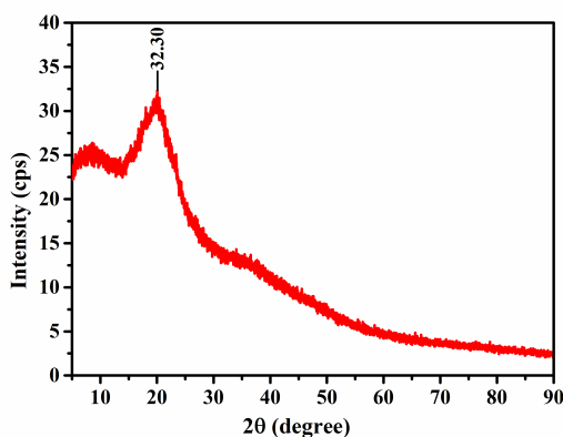
Graph2: XRD Spectra of Soup stick powder. Where X= 2θ and y= intensity (a.u.).
