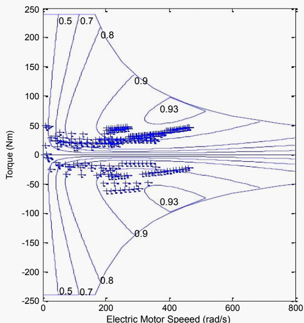
Figure 14: Motor operation points with four gear ratios.
