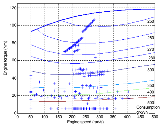
Figure 6: Engine operation points, NEDC cycle- traditional ICE vehicle.
