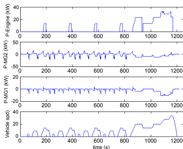
Figure 8: Power flows in the HEV with the twin epicyclic gearbox over NEDC driving cycle.
