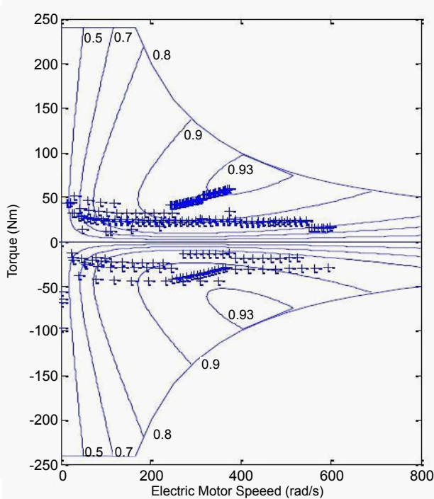
Figure 15: Motor operation points with two gear ratios.
