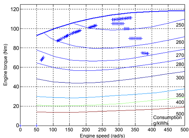
Figure 7: Engine operation points, NEDC cycle- twin epicyclic system.
