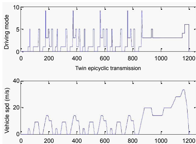
Figure 9: Mode selection- Europe NEDC cycle.
