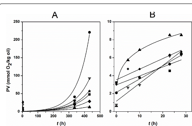
Figure 3: Peroxide value (PV) determined for the studied oils at moderate (A; 65°C) and elevated (B; 180°C) temperatures. Legend: ■ AR; ● CH; ★ RM; ▲ OL; ▼ RS; ◆ SF.
