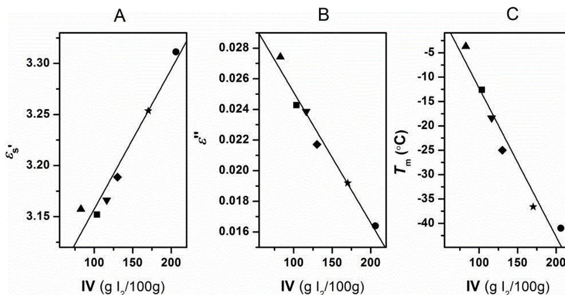
Figure 2: Dependence of the static dielectric constant ( \epsilon'_s ), dielectric loss (2 MHz) ( \epsilon'' ) and melting temperature ( T_m ) of the studied oils on iodine value (IV). Legend: ■ AR; ● CH; ★ RM; ▲ OL; ▼ RS; ◆ SF.
