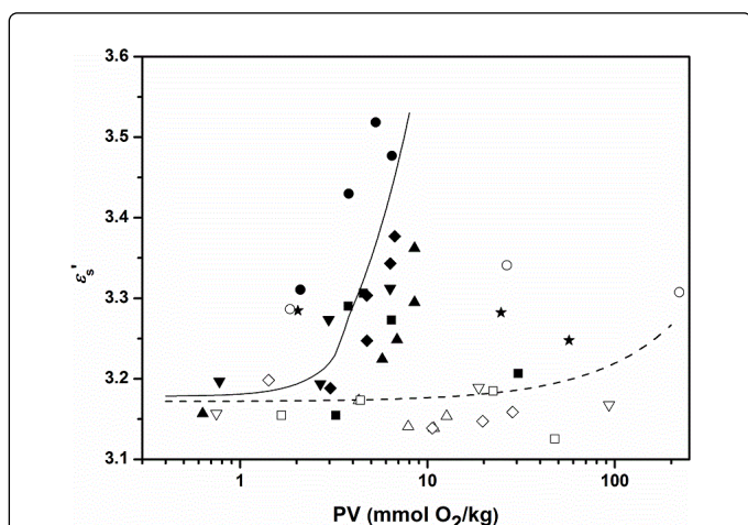
Figure 5: Dependence of static dielectric constant ( \epsilon'_s ) on peroxide value (PV) for oils treated at 65°C (- - -) for 432 hr and at 180°C for 28 hr (-). Legend: □AR 65°C; ○CH 65°C; △OL 65°C; ★RM 65°C; ▼RS 65°C; ◆SF 65°C; ■AR 180°C; ●CH 180°C; ▲OL 180°C; ▼RS 180°C; ◆SF 180°C.
