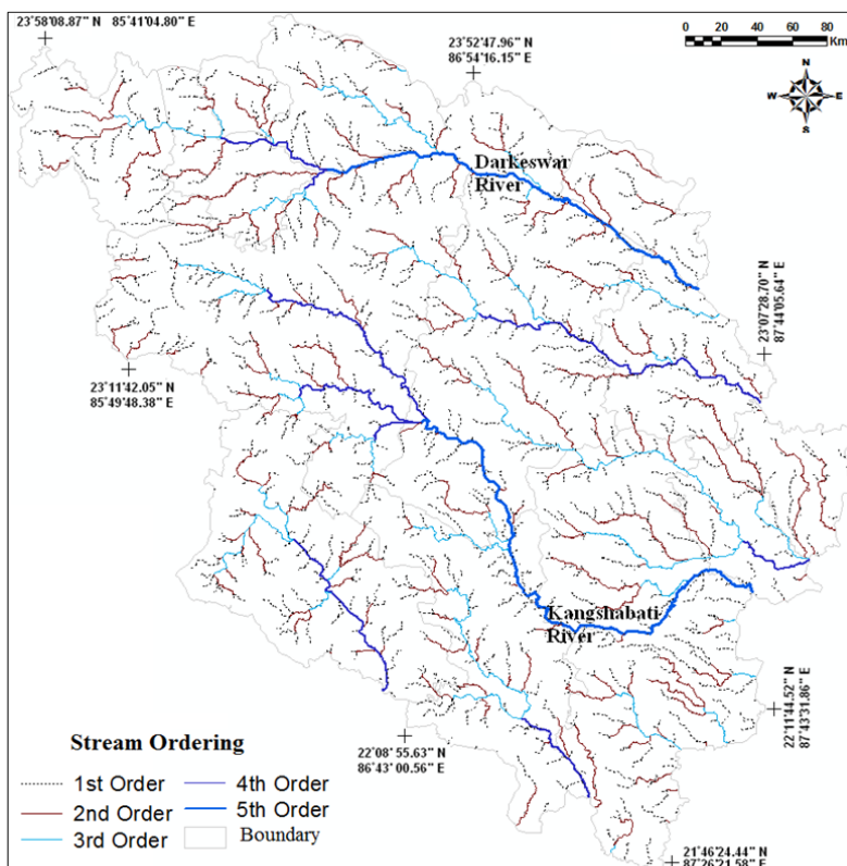
Figure 6: Stream Ordering of the Kangshabati-Darkeswar Interfluves Area.
