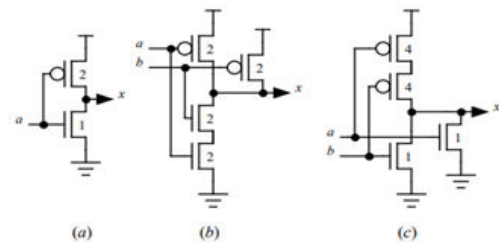
Fig.3.1: a) Inverter b) 2-input NAND Gate c) 2-input NOR Gate
