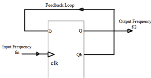
Figure.4.2: Binary Counter
