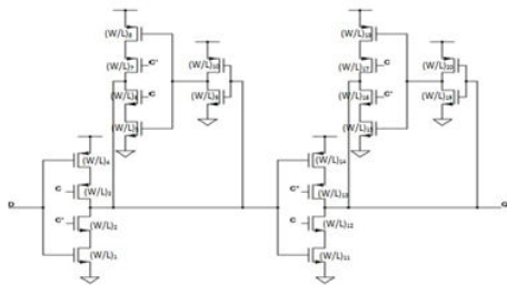
Figure.4.1: C2MOS D flip flop structure
