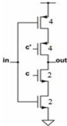
Figure.2.2: The Clocked inverter
