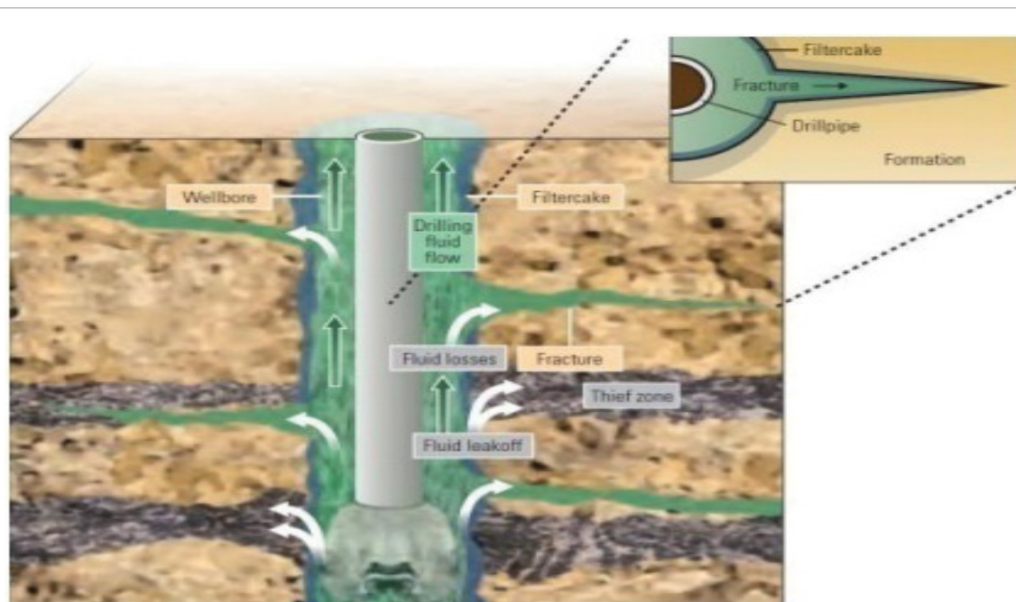
Figure 1: Schematic illustration of formation of cracks during petroleum drilling operations.
