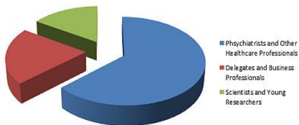
Participation Ratio
