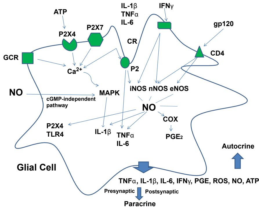
Figure 2: Activated glial cell produces neuroactive mediator and responds to neuroactive mediator with special references to NO. Glial cell is activated by inflammatory mediators, bacteria, virus, and nerve injury. Nerve injury produces ATP from presynaptic neuron and activates glial cells. NO comes from postsynaptic neuron in persistent pain state and activates glia through MAPK activation (Figure 1). Activated glia reduces uptake of glutamate, increasing synaptic glutamate concentration, intensifying pain. IL-1,IL-6, TNF \alpha , IFN \gamma , and gp120 induces NO production via NOS with subsequent increase in IL-1,IL-6, TNF \alpha ,IFN \gamma , and PGE2, working on itself, neighboring glia and neurons with autocrine and paracrine manner.
