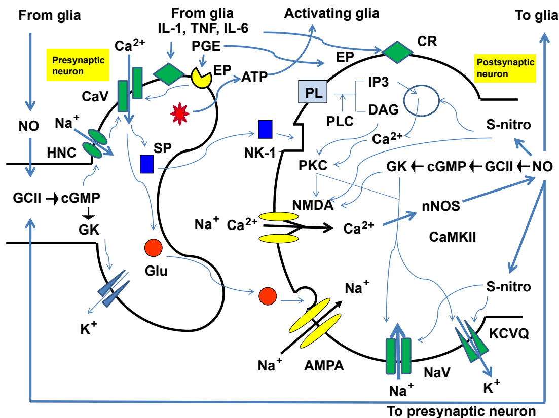
Figure 1: Postsynaptic NMDA-NOS-NO pathway enhances presynaptic glutamate release and postsynaptic transmission, and activates glia in persistent pain. In acute pain, glutamate, SP, and ATP are released from the presynaptic neuron. Glutamate activates AMPA receptor and induces excitatory postsynaptic potential, which opens NaV causing action potential. Once the acute noxious stimuli and inflammatory response has gone, the pain would disappear. When repetitive noxious stimulation continues, SP activates NK-1 receptor, causing PLC activation making IP3 and DAG from phospholipid. IP3 stimulates Ca 2+ release from Ca 2+ stored site. Increased Ca 2+ and DAG activates C kinase which phosphorylates NMDA receptor with subsequent Ca 2+ and Na + influx into the postsynaptic secondary neuron, followed by activation of nNOS, NO production, Guanylyl cyclase activation, cGMP formation, activation of GK, inducing the further activation of NMDA receptor. NO produced in the secondary neuron diffuses out of the neuron and reach the presynaptic neuron and neighboring glial cell. In the presynaptic neuron NO-induced GK activation closes K channel with its phosphorylation and opens HNC, causing depolarization with subsequent activation of Ca 2+ channel. Increase in Ca 2+ releases the glutamate and SP into the synaptic cleft causing vicious cycle.
