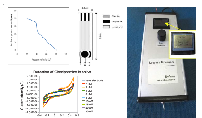
Figure 5: (above, left) Langmuir \pi -A isotherm of the recombinant laccase thin film [36,39] and screen-printed electrodes based on graphite/ruthenium ink and on silver one; (below, left) cyclic voltammetry (CV) of laccase-based biosensor for detection of clomipramine at increasing concentrations in saliva; (right) prototype of laccase sensor, compact and portable for different biological fluids. The shown CV is routinely applied for the analysis of water contaminants, such as phenols and phenolic derivatives and compounds with our device and other ones [40,41].
