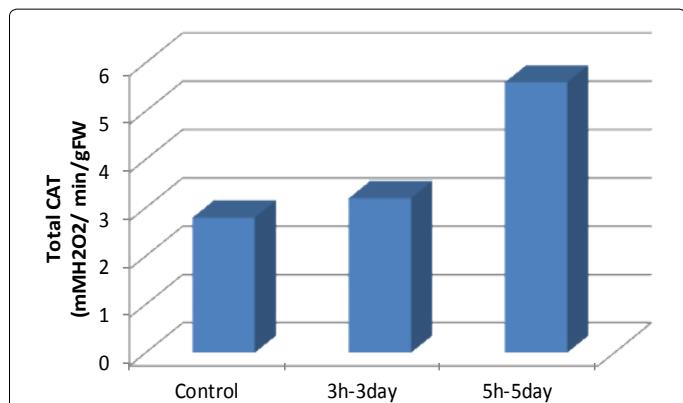
Figure 5: Effect of RF (GSM) and Mobile phone-940 MHz on the activity of catalase ( p < 0.05 by Duncan's test).
