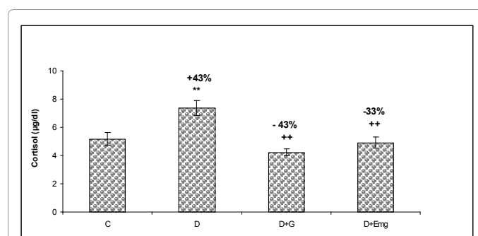
Figure 5: Cortisol (µg/dl) level after 4 weeks in control, diabetic and treated diabetic rats.
