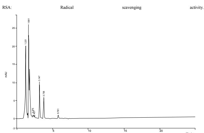
Figure 7: HPLC profile of phenolic acids ( \lambda=230 nm) from garlic aqueous extract.
