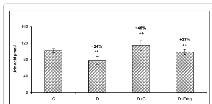
Figure 4: Uric acid (µmol/l) level after 4 weeks in control, diabetic and treated diabetic rats.
