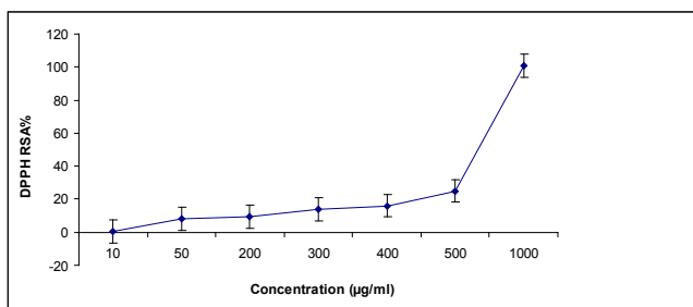
Figure 6: Scavenging activity of garlic extract (at final concentration ranging from 10 to 1000 µg/ml) upon the DPPH radical.
