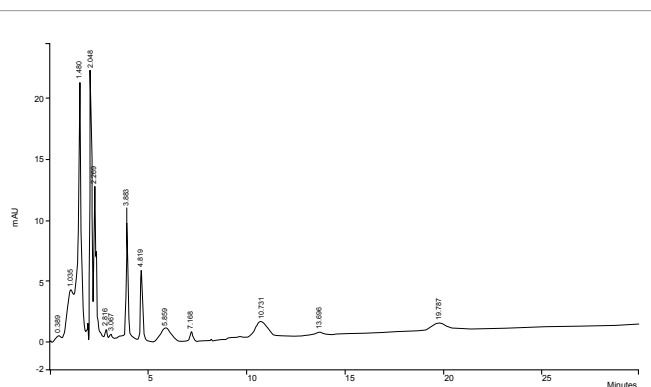
Figure 8: HPLC profile of flavonoids ( \lambda=365 nm) from garlic aqueous extract.
