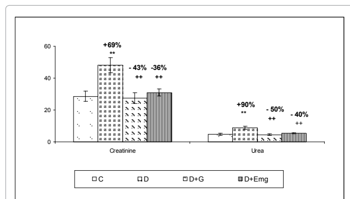
Figure 2: Serum creatinine (μmol/l) and urea (mmol/l) levels after 4 weeks in control, diabetic and treated diabetic rats.
