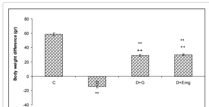
Figure 1: Comparison of body weight after 4 weeks of treatment in control, diabetic and treated diabetic rats. The mean weight of all animals was 160 g when starting the experiments
