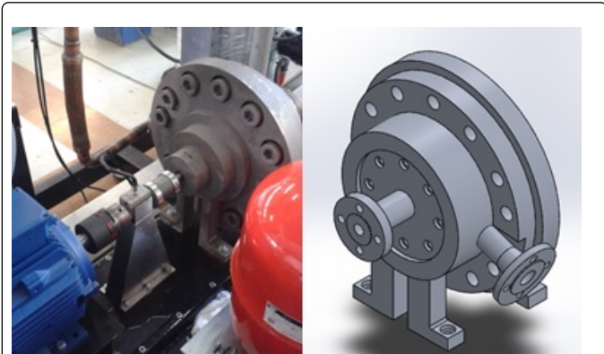
Figure 2: Left hand side: Scroll expander coupled with asynchronous motor/generator. Right hand side: Design of open-drive scroll expander.
