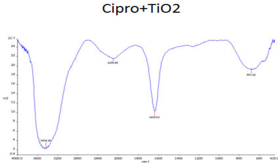
Figure5: FTIR results of Ciprofloxacin with TiO 2 nanoparticles
