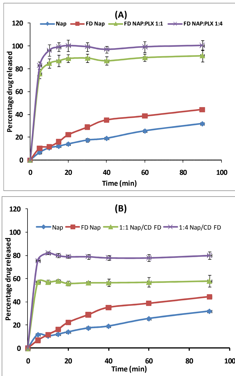
Figure 2: Percentage drug released from pure untreated drug (Nap) and freeze dried drug (FD Nap) and binary formulations with poloxamer 407 (A) and \beta -cyclodextrin (B).
