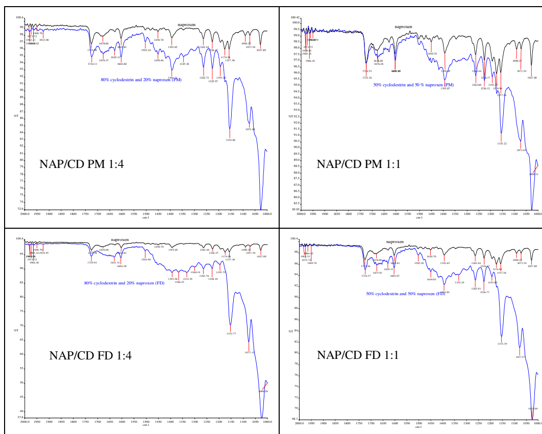
Figure 4: FT-IR spectra of naproxen formulations
