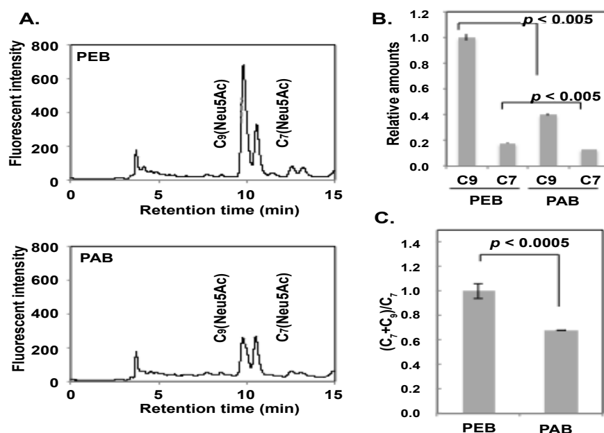
Figure 4: Fluorometric C_7/C_9 analysis. The PEB and PAB crude samples (100 \mu g as BSA) were treated with monoSia-specific sialidase, electrophoresed and blotted onto PVDF membrane. PolySia-NCAM at greater than 100 kDa area were cut out and subjected to fluorometric C_7/C_9 analysis. The samples were treated with mild periodate and non-reducing terminal end of \alpha -2,8-linked oligo/polySia was changed to C_7 -analogues while internal sialic acid ( C_9 -sialic acid) remain unchanged. After acid treatment, C_7 - and C_9 -Sias were released and labeled with DMB. The DMB-labeled sialic acids were applied to the HPLC equipped with a Wako Handy ODS column (250 \times 4.6 mm, Wako), and a fluorescence detector (FP-2025, JASCO). The column is equilibrated using methanol/acetonitrile/water (7:9:84, v/v/v) at 26 ^{\circ} C. Samples were applied to HPLC analysis isocratically flow at 1.0 ml/min. (A) Typical chromatograms of C_7/C_9 analysis of PEB and PAB samples. (B) Relative amounts of C_9 -Neu5Ac and C_7 -Neu5Ac derived from PEB and PAB samples. The amount of C_9 -Neu5Ac derived from PEB was set equal to 1.0. (C) The (C_7+C_9)/C_7 index. The index of PEB was set to 1.0.
