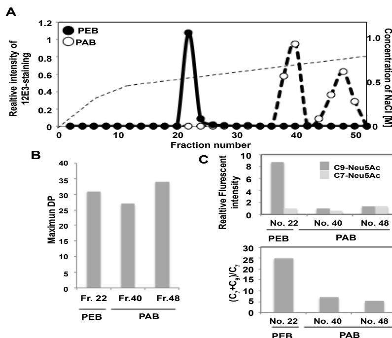
Figure 5: Mono Q anion exchange chromatography of PEB and PAB. PEB and PAB were treated with monoSia-specific sialidase and subjected to the mono Q anion exchange chromatography. The samples were eluted with a NaCl gradient (0-10 min, 0 M; 10-30 min, 0 \rightarrow 0.3 M; 30-105 min, 0.3 \rightarrow 0.5 M; 105-135 min, 0.5 \rightarrow 3 M) in 20 mM Tris-HCl (pH 8.0). The flow rate was 0.5 ml/min and 1 ml was collected per fraction. After the samples were dot-blotted onto a PVDF membrane, the amount of polySia in each fraction was determined by the anti-polySia staining (12E3) of the membrane. (A) Chromatogram of mono Q anion exchange chromatography. (B) MH-FAEC analysis of peaks detected with 12E3 staining, fraction (fr.) 22 from PEB and fr. 40 and 48 from PAB. Maximum DP of the samples were shown. (C) Fluorometric C_7/C_9 analysis. Upper panel shows relative amounts of C_7 -Neu5Ac and C_9 -Neu5Ac. Samples derived from peaks detected with 12E3 staining, fraction 22 from PEB and fraction 40 and 48 from PAB were analyzed. Lower panel shows the (C_7+C_9)/C_7 value, index as quality of di/oligo/polySia.
