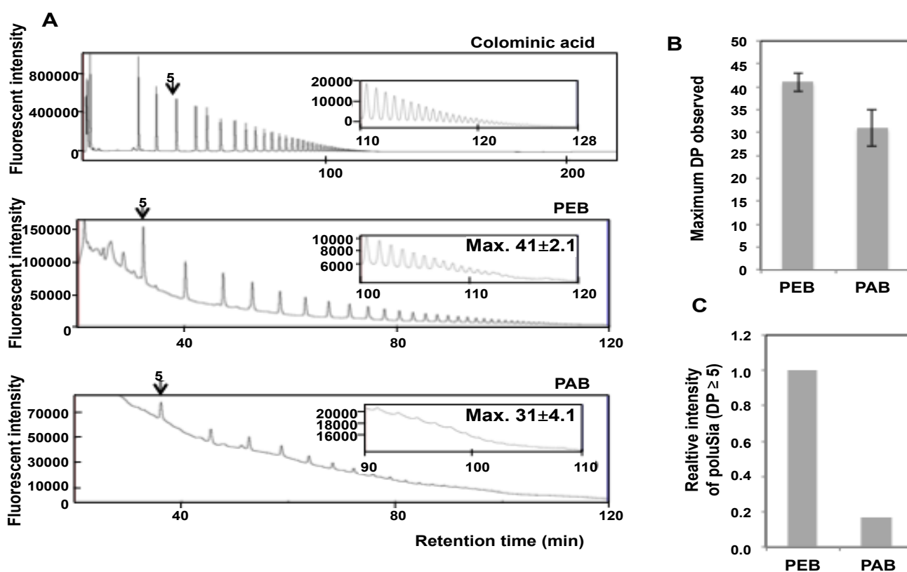
Figure 3: Mild acid hydrolysis-fluorometric anion-exchange chromatography analysis (MH-FAEC). The PEB and PAB crude samples (1 mg as BSA) were mild acid hydrolyzed and simultaneously labeled with DMB. Released and labeled oligo/polySias were separated with DNA-Pac PA-100 anion exchange chromatography and eluted with a gradient of NaCl (0-15 min, 0 M; 15-185 min, 0 → 0.6 M; 185-190 min, 0.6 → 1.0 M) in 20 mM Tris-HCl (pH 8.0). The flow rate was 1 ml/min. Eluted oligo/polySia-DMBs were monitored with fluorescent detector (Ex 373 nm, Em 448 nm). (A) Chromatograms of MH-FAEC. Colominic acid, PEB and PAB were analyzed. Three independent experiments were performed and typical chromatograms were shown. The average of Maximum DP (B) and the relative amounts of oligo/polySia ((Neu5Ac) n-DMB, n ≥ 6) obtained by three independent experiments. The sum of intensity of oligo/polySia (Neu5Ac) n-DMB, n ≥ 6) was set to 1.0.
