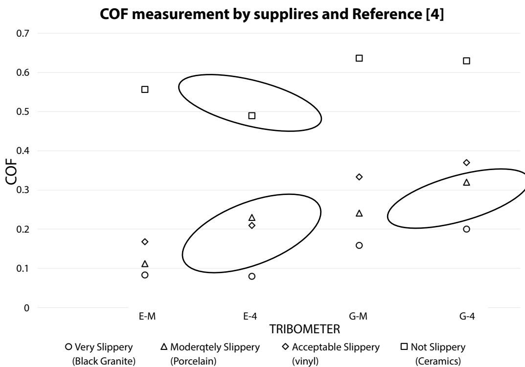
Figure 4: Manufacturers' tests results compared to the results in [4]. (E-M – Tribometer E - supplier's results; E-4 - Tribometer E - Ref. 4 results; G-M – Tribometer G - supplier's results; G-4 - Tribometer G - Ref. 4 results)
