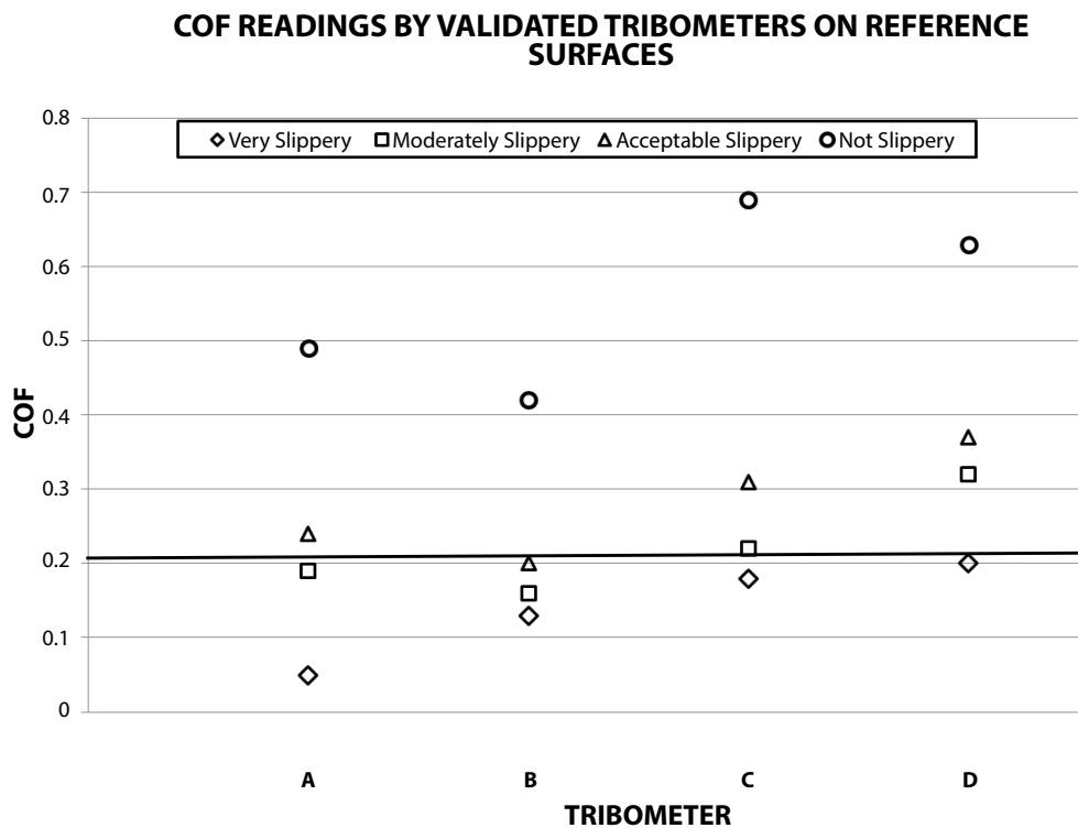
Figure 1: COF measurements of the reference surfaces by the 4 validated tribometers.
