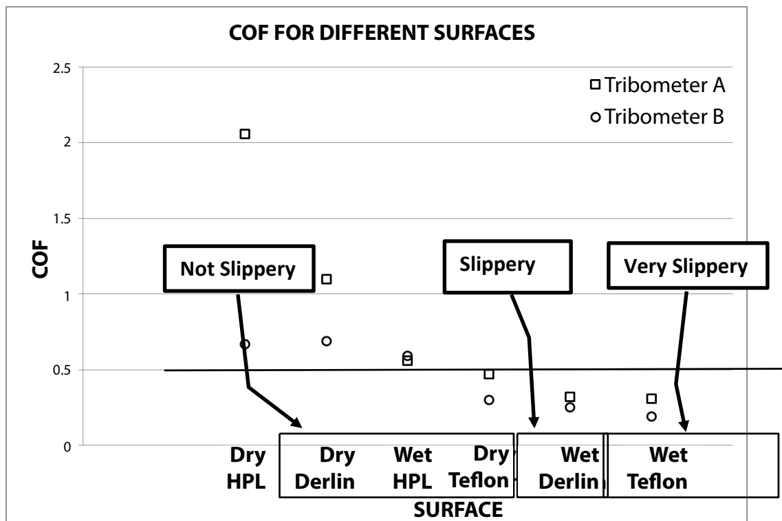
Figure 2: COF measurements of the reference surfaces by the 2 validated tribometers.
