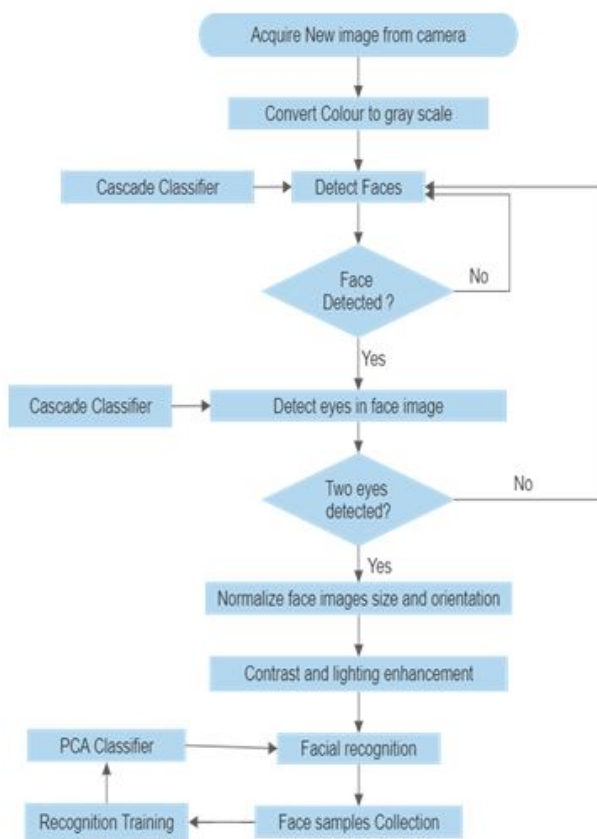
Figure 2: Proposed Flow Diagram
