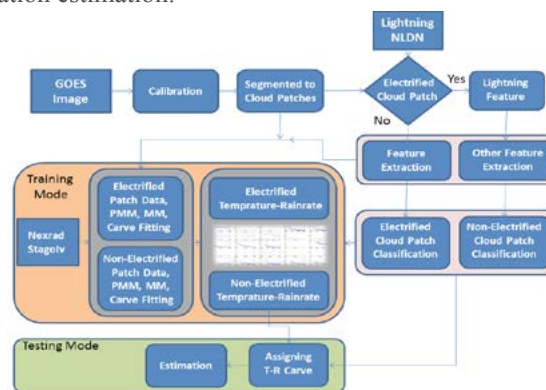
Figure 1: High resolution satellite precipitation estimation block diagram
