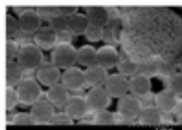
Figure 1: Scanning electron microscope image of spheres-on-sphere silica particles. The inset shows one SOS particle.
