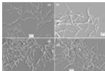
SEM micrographs of NCC: cotton linters (a), chinese silver grass (b), spruce wood (c) and eucalyptus wood (d).
