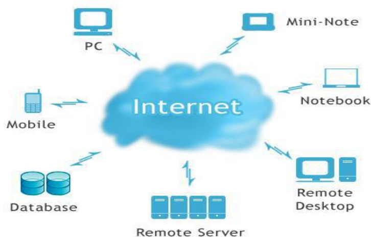
Fig. 1 Cloud Computing
